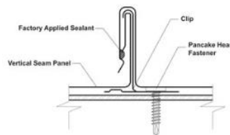
ATTACHMENT DETAIL
